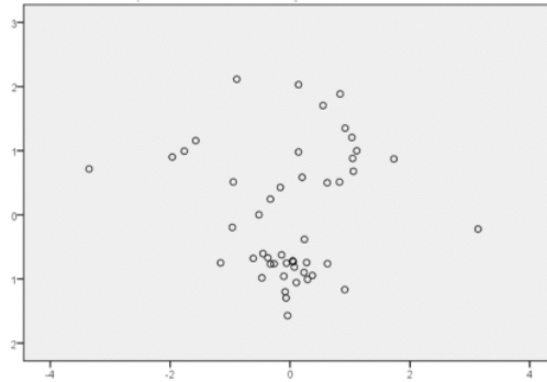
Figure 8. Scatter Plots
