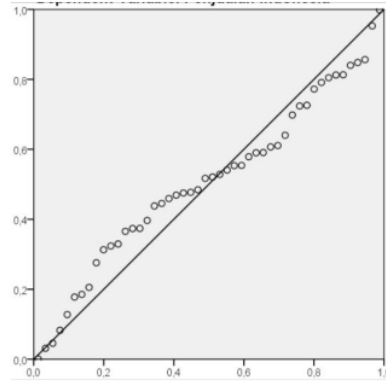
Figure 7. Normal PP Plot
