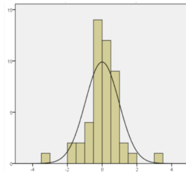
Figure 6. Histogram Chart
