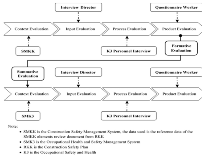
Figure 1. Conceptual framework
