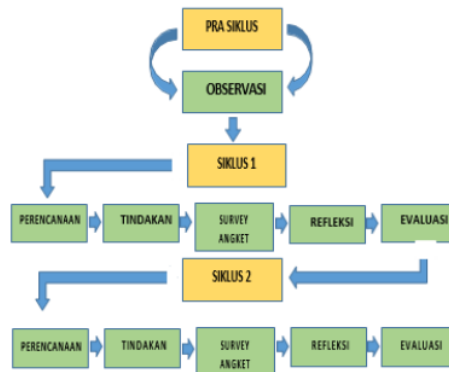
Gambar 2.1 Prosedur Penelitian
