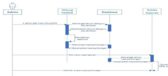
Gambar 4. Sequence Diagram Login
