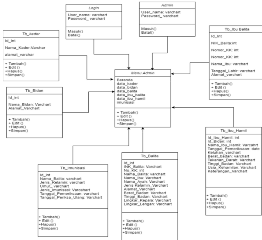
Gambar 2.5 Class Diagram
