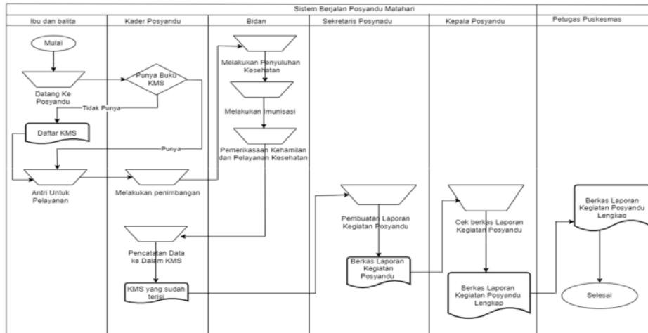
Gambar flowchart
