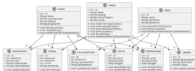
Gambar 4.2 Class Diagram
