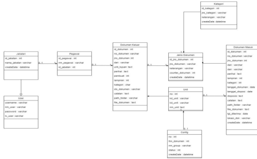
Gambar 3 Class Diagram Alur input Output Data
