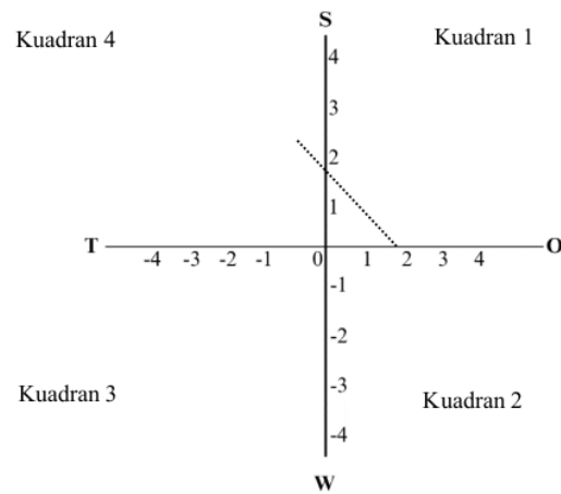
Gambar 1 Diagram SWOT
