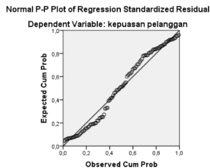
Gambar 1. Grafik Normal Probability Plot (P-Plot)
